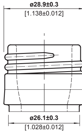
FINISH DETAIL - 2:1
