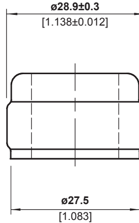
FINISH DETAIL - 2:1
