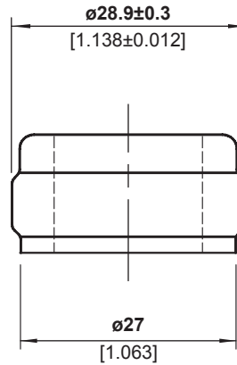
FINISH DETAIL - 2:1
