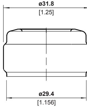
FINISH DETAIL - 2:1
