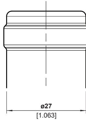
FINISH DETAIL - 2:1
