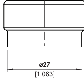
FINISH DETAIL - 2:1
