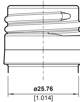
FINISH DETAIL - 2:1
