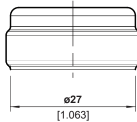
FINISH DETAIL - 2:1
