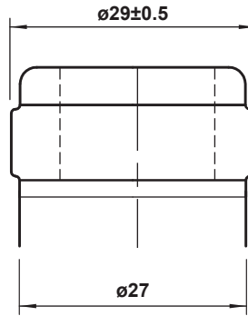
FINISH DETAIL - 2:1
