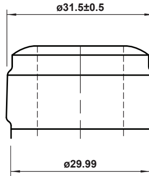
FINISH DETAIL - 2:1
