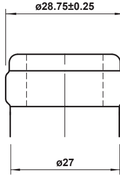
FINISH DETAIL - 2:1
