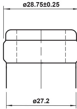
FINISH DETAIL - 2:1
