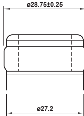
FINISH DETAIL - 2:1
