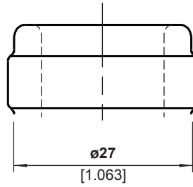
FINISH DETAIL - 2:1
