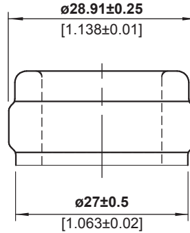
FINISH DETAIL - 2:1
