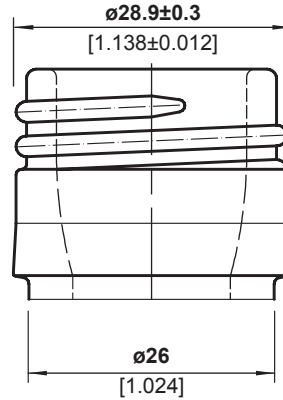
FINISH DETAIL - 2:1
