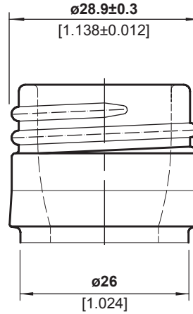
FINISH DETAIL - 2:1
