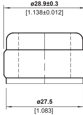
FINISH DETAIL - 2:1
