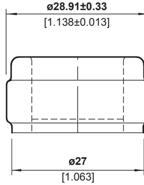
FINISH DETAIL - 2:1
