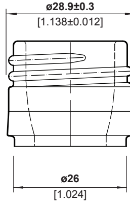
FINISH DETAIL - 2:1
