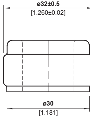
FINISH DETAIL - 2:1
