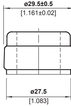
FINISH DETAIL - 2:1
