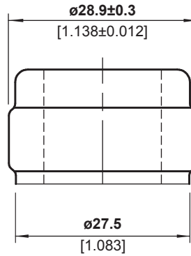
FINISH DETAIL - 2:1
