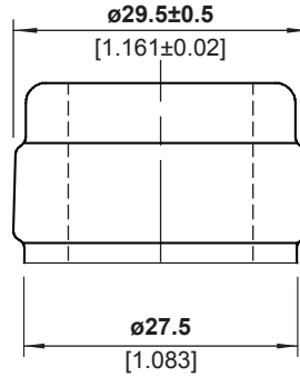
FINISH DETAIL - 2:1
