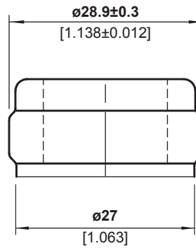
FINISH DETAIL - 2:1
