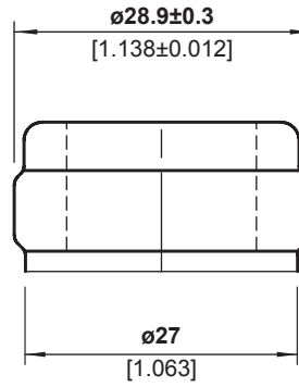
FINISH DETAIL - 2:1
