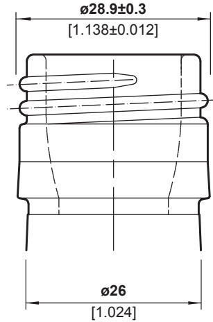
FINISH DETAIL - 2:1
